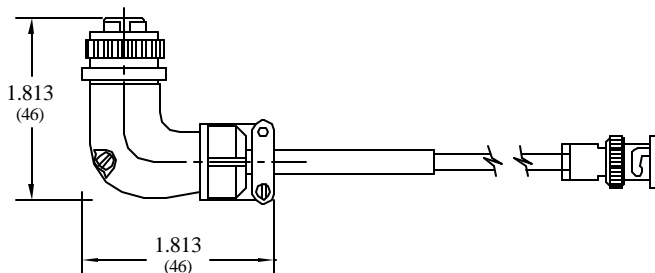
RIGHT ANGLE CONNECTOR W/BNC CONNECTOR
