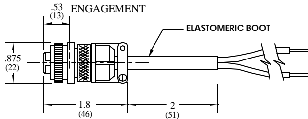
STRAIGHT CONNECTOR W/STRIPPED LEADS
